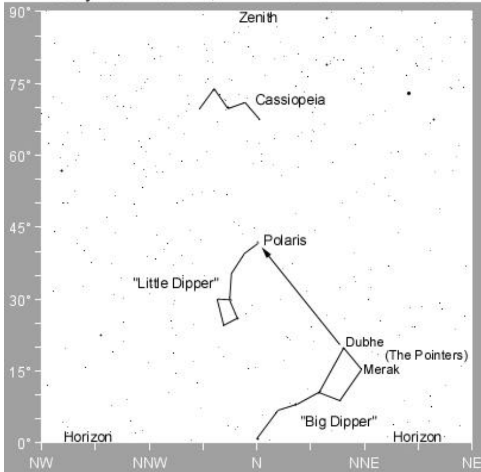
The Sky from Bedford, NY 17:45 EST 19 JAN 2005
