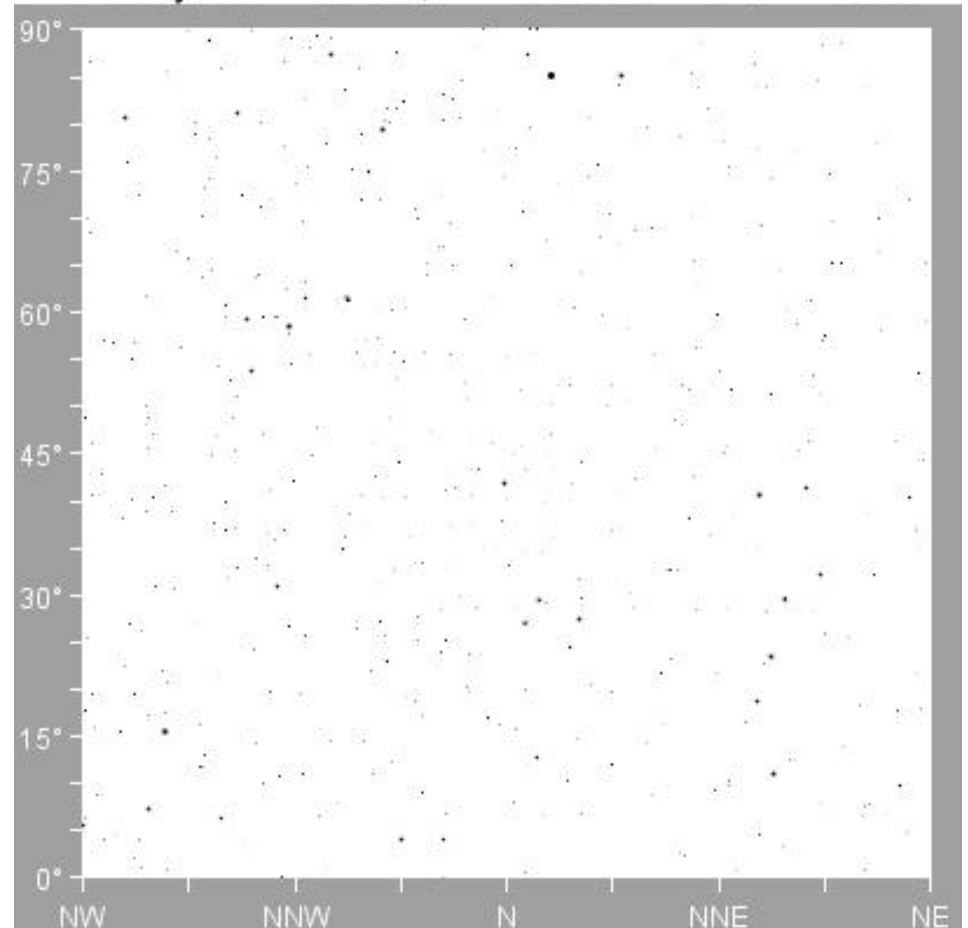
The Sky from Bedford, NY 20:45 EST 19 JAN 2005
